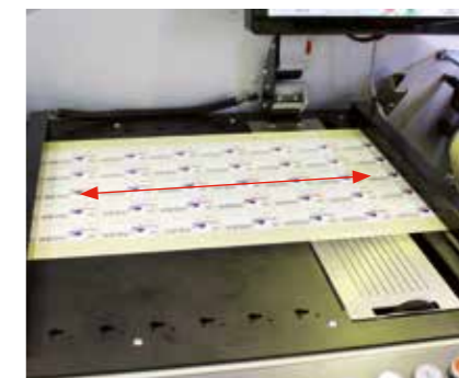
Moveable web clamps allow for easy replacement of long or short labels
